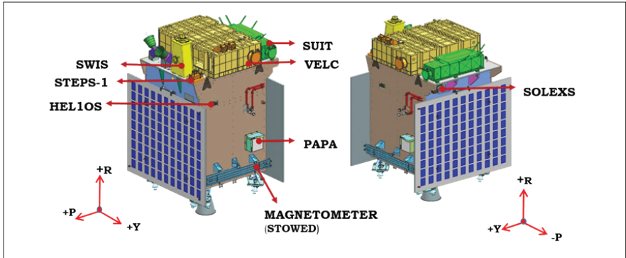
Fig1: Locations of Aditya-L1 payloads on the spacecraft. R, P and Y indicate the Raw, Pitch and Roll axis of the spacecraft. ASPEX Payload Consists of SWIS & STEPS.
