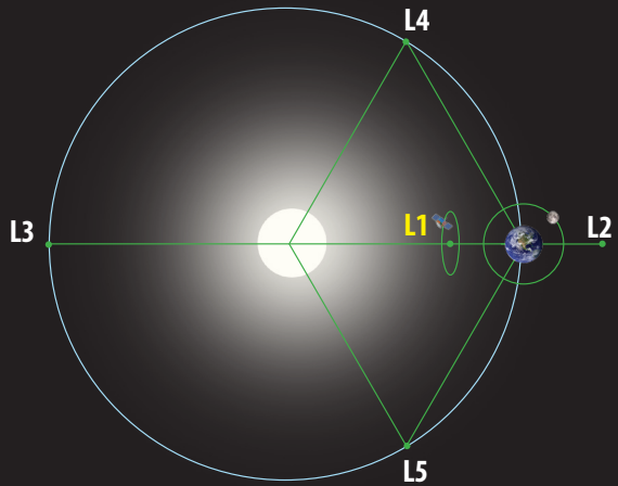
Fig 2 : Illustration of Lagrange points of the Sun-Earth system
