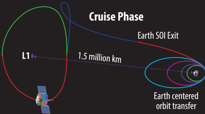
Fig 3: Aditya-L1 trajectory from Earth to L1.
